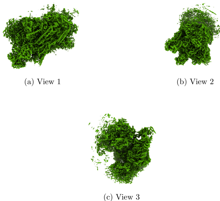
Figure 4: Isosurface at threshold=0.028100. Views generated by ChimeraX at a the following X, Y, Z angles: View 1 (0, -90, -90), View 2 (-90, 0, -90), View 3 (0, 0, 0).
