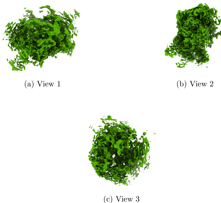
Figure 4: Isosurface at threshold=0.018200. Views generated by ChimeraX at a the following X, Y, Z angles: View 1 (0, -90, -90), View 2 (-90, 0, -90), View 3 (0, 0, 0).
