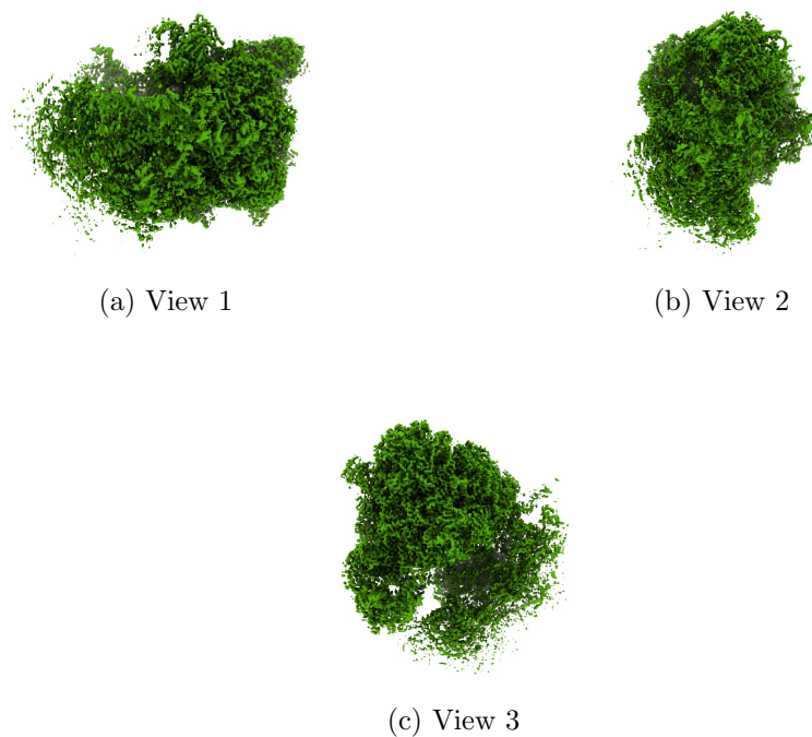
Figure 4: Isosurface at threshold=0.043900. Views generated by ChimeraX at a the following X, Y, Z angles: View 1 (0, -90, -90), View 2 (-90, 0, -90), View 3 (0, 0, 0).
