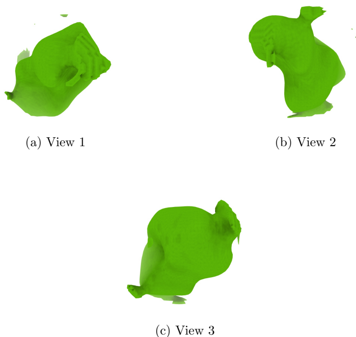
Figure 4: Isosurface at threshold=3.320000. Views generated by ChimeraX at a the following X, Y, Z angles: View 1 (0, -90, -90), View 2 (-90, 0, -90), View 3 (0, 0, 0).
