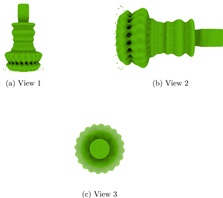
Figure 4: Isosurface at threshold=0.022700. Views generated by ChimeraX at a the following X, Y, Z angles: View 1 (0, -90, -90), View 2 (-90, 0, -90), View 3 (0, 0, 0).
