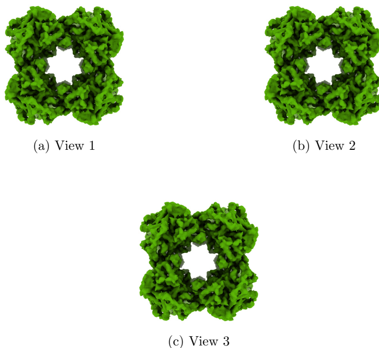
Figure 4: Isosurface at threshold=0.023300. Views generated by ChimeraX at a the following X, Y, Z angles: View 1 (0, -90, -90), View 2 (-90, 0, -90), View 3 (0, 0, 0).
