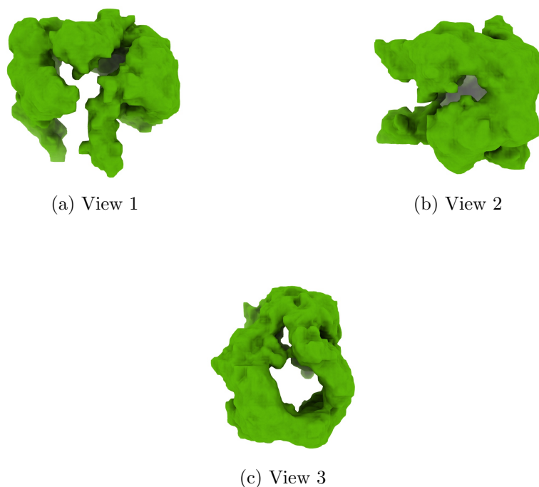
Figure 4: Isosurface at threshold=1.990000. Views generated by ChimeraX at a the following X, Y, Z angles: View 1 (0, -90, -90), View 2 (-90, 0, -90), View 3 (0, 0, 0).
