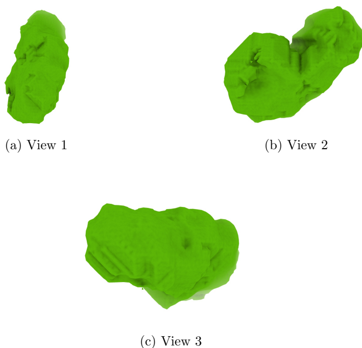
Figure 4: Isosurface at threshold=0.607000. Views generated by ChimeraX at a the following X, Y, Z angles: View 1 (0, -90, -90), View 2 (-90, 0, -90), View 3 (0, 0, 0).
