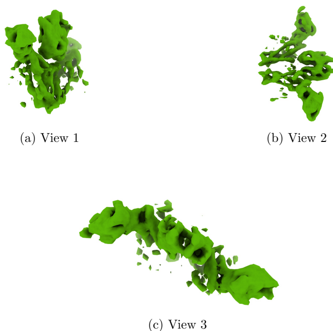
Figure 4: Isosurface at threshold=0.268000. Views generated by ChimeraX at a the following X, Y, Z angles: View 1 (0, -90, -90), View 2 (-90, 0, -90), View 3 (0, 0, 0).
