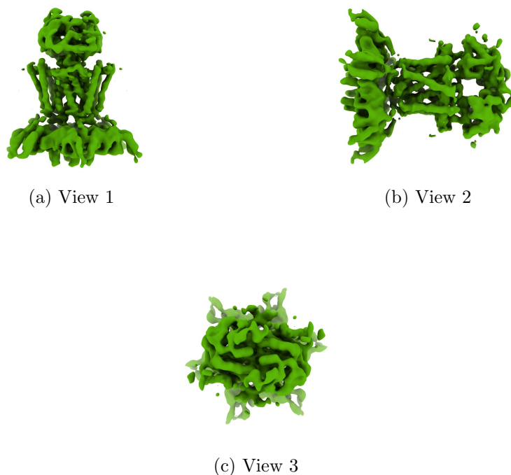
Figure 4: Isosurface at threshold=0.057600. Views generated by ChimeraX at a the following X, Y, Z angles: View 1 (0, -90, -90), View 2 (-90, 0, -90), View 3 (0, 0, 0).
