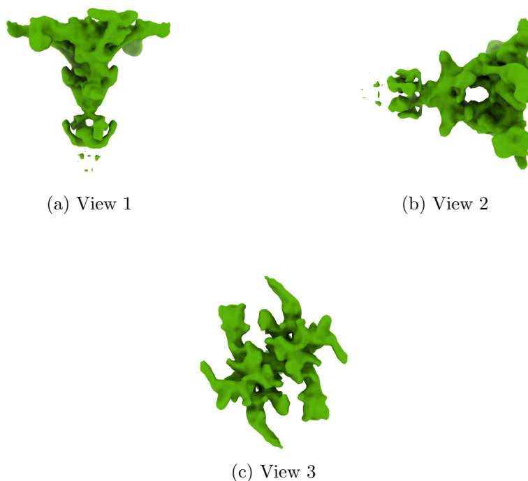
Figure 4: Isosurface at threshold=0.509000. Views generated by ChimeraX at a the following X, Y, Z angles: View 1 (0, -90, -90), View 2 (-90, 0, -90), View 3 (0, 0, 0).
