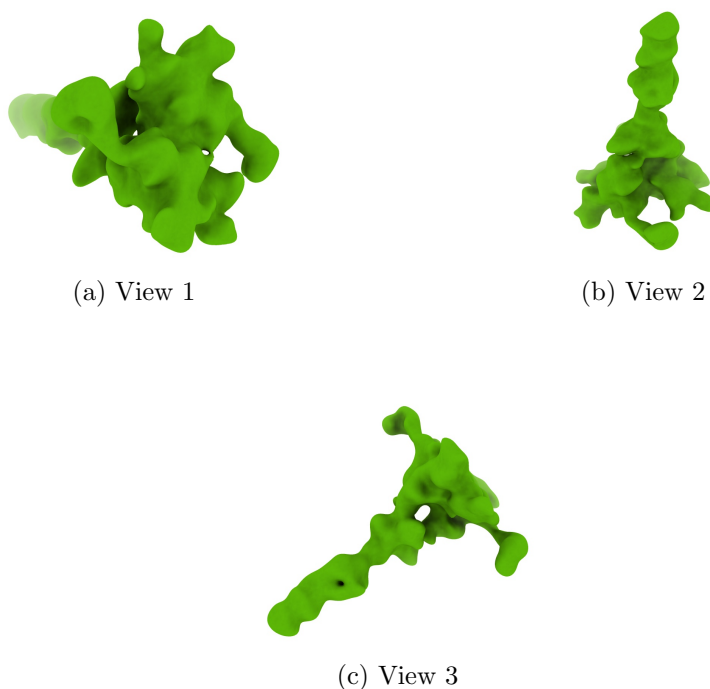
Figure 4: Isosurface at threshold=0.034100. Views generated by ChimeraX at a the following X, Y, Z angles: View 1 (0, -90, -90), View 2 (-90, 0, -90), View 3 (0, 0, 0).
