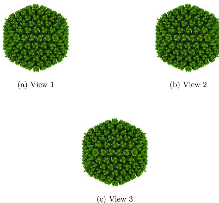
Figure 4: Isosurface at threshold=180.000000. Views generated by ChimeraX at a the following X, Y, Z angles: View 1 (0, -90, -90), View 2 (-90, 0, -90), View 3 (0, 0, 0).
