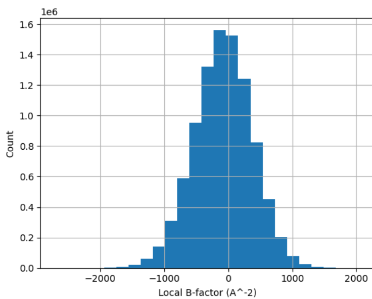
Figure 10: Histogram of the local B-factor according to LocBfactor.
