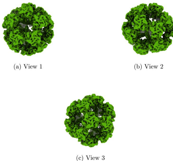
Figure 4: Isosurface at threshold=0.023500. Views generated by ChimeraX at a the following X, Y, Z angles: View 1 (0, -90, -90), View 2 (-90, 0, -90), View 3 (0, 0, 0).
