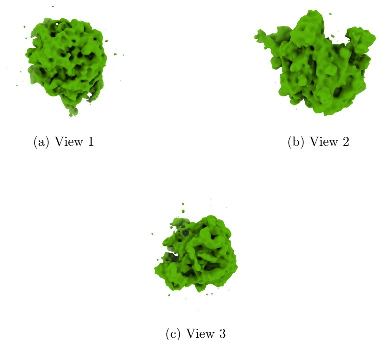
Figure 4: Isosurface at threshold=55.300000. Views generated by ChimeraX at a the following X, Y, Z angles: View 1 (0, -90, -90), View 2 (-90, 0, -90), View 3 (0, 0, 0).
