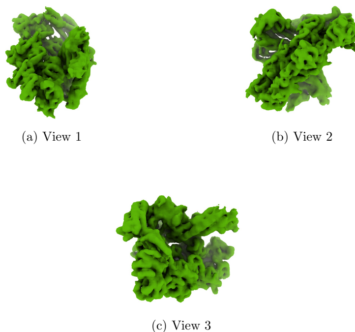
Figure 4: Isosurface at threshold=0.035300. Views generated by ChimeraX at a the following X, Y, Z angles: View 1 (0, -90, -90), View 2 (-90, 0, -90), View 3 (0, 0, 0).
