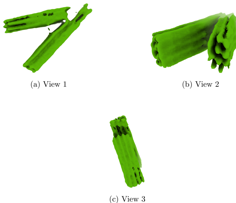
Figure 4: Isosurface at threshold=0.069000. Views generated by ChimeraX at a the following X, Y, Z angles: View 1 (0, -90, -90), View 2 (-90, 0, -90), View 3 (0, 0, 0).
