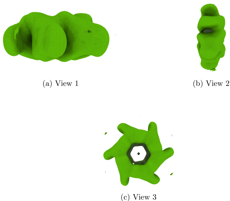
Figure 4: Isosurface at threshold=0.002920. Views generated by ChimeraX at a the following X, Y, Z angles: View 1 (0, -90, -90), View 2 (-90, 0, -90), View 3 (0, 0, 0).
