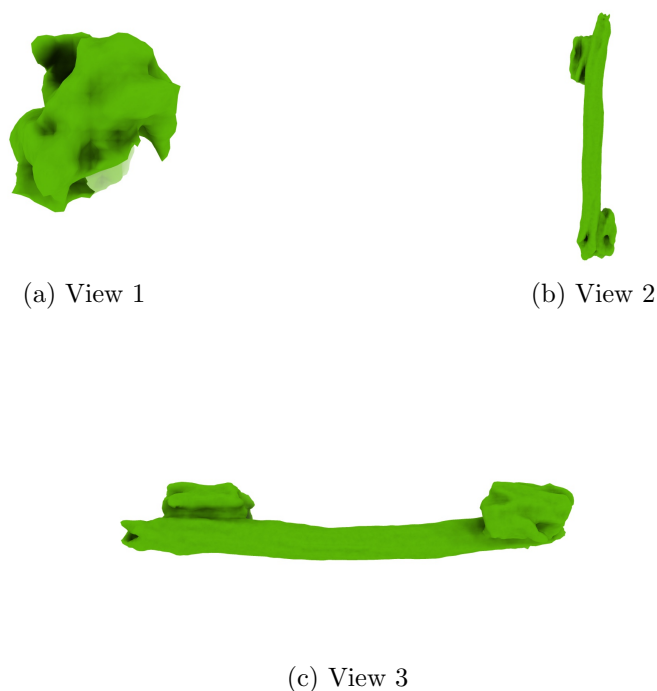
Figure 4: Isosurface at threshold=0.050000. Views generated by ChimeraX at a the following X, Y, Z angles: View 1 (0, -90, -90), View 2 (-90, 0, -90), View 3 (0, 0, 0).
