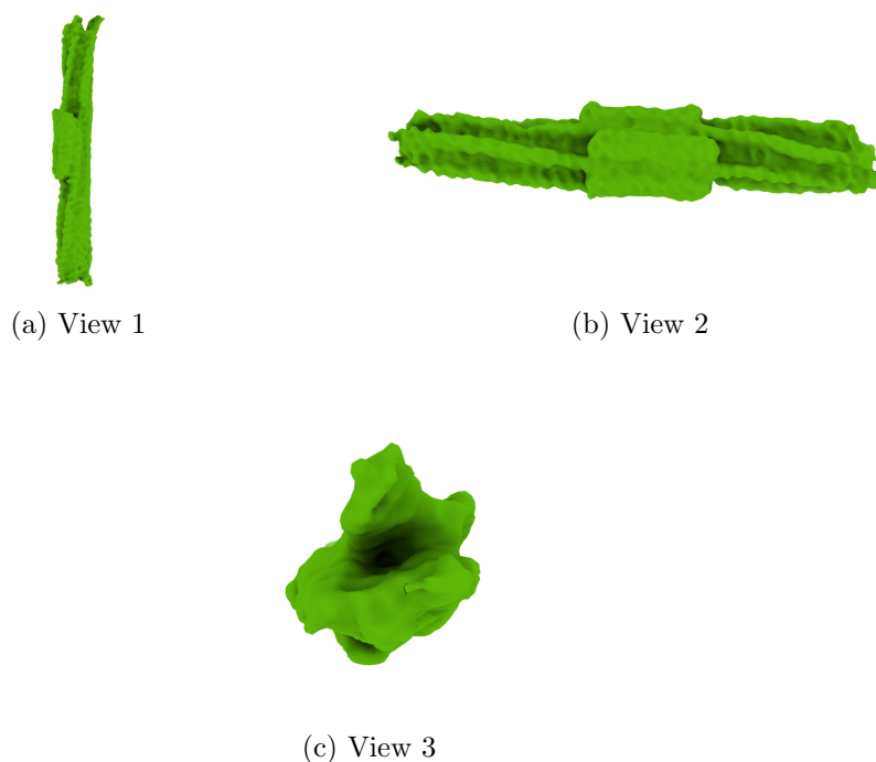
Figure 4: Isosurface at threshold=0.048000. Views generated by ChimeraX at a the following X, Y, Z angles: View 1 (0, -90, -90), View 2 (-90, 0, -90), View 3 (0, 0, 0).
