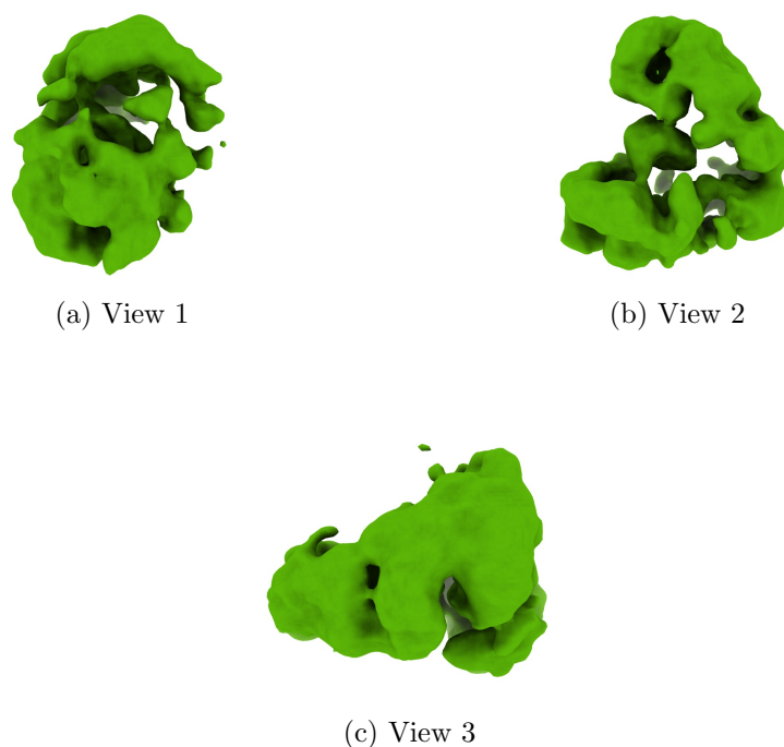
Figure 4: Isosurface at threshold=0.169000. Views generated by ChimeraX at a the following X, Y, Z angles: View 1 (0, -90, -90), View 2 (-90, 0, -90), View 3 (0, 0, 0).
