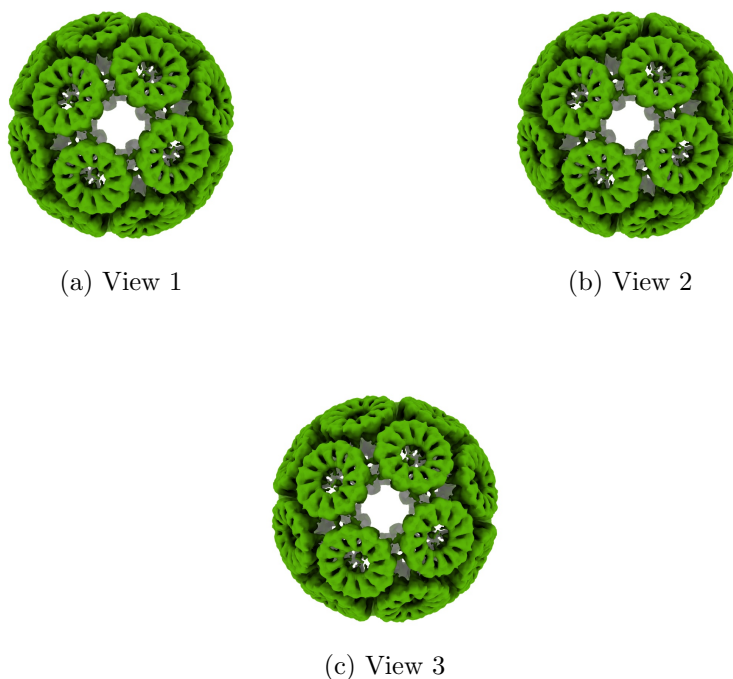
Figure 4: Isosurface at threshold=1.780000. Views generated by ChimeraX at a the following X, Y, Z angles: View 1 (0, -90, -90), View 2 (-90, 0, -90), View 3 (0, 0, 0).
