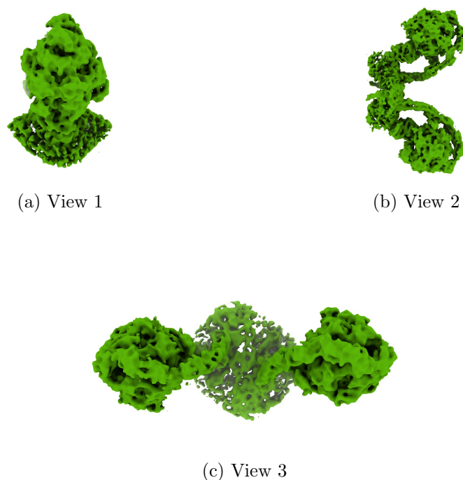
Figure 4: Isosurface at threshold=0.013200. Views generated by ChimeraX at a the following X, Y, Z angles: View 1 (0, -90, -90), View 2 (-90, 0, -90), View 3 (0, 0, 0).
