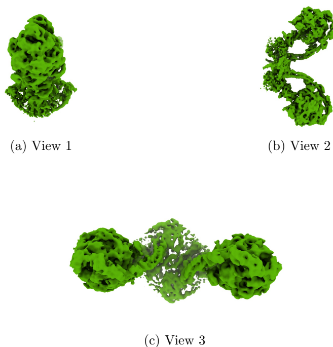
Figure 4: Isosurface at threshold=0.014600. Views generated by ChimeraX at a the following X, Y, Z angles: View 1 (0, -90, -90), View 2 (-90, 0, -90), View 3 (0, 0, 0).
