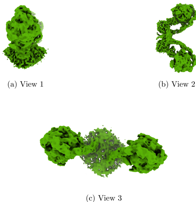
Figure 4: Isosurface at threshold=0.012400. Views generated by ChimeraX at a the following X, Y, Z angles: View 1 (0, -90, -90), View 2 (-90, 0, -90), View 3 (0, 0, 0).
