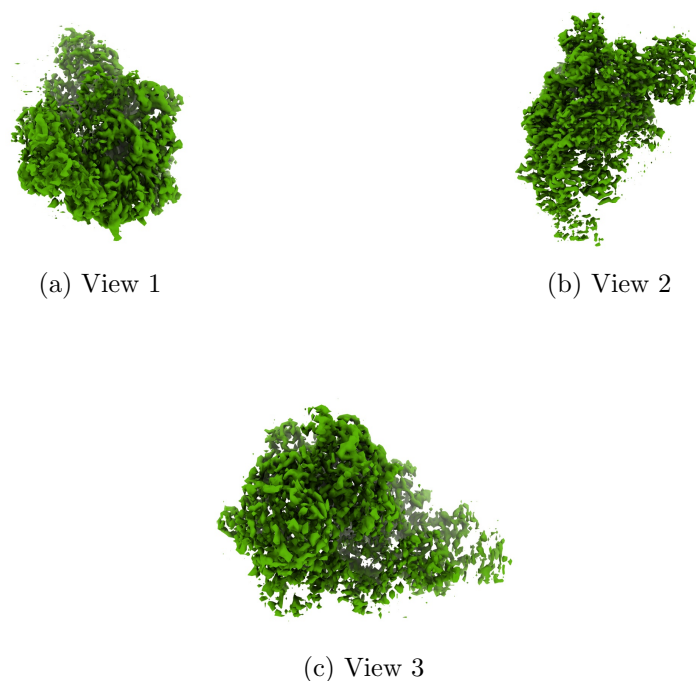
Figure 4: Isosurface at threshold=0.015300. Views generated by ChimeraX at a the following X, Y, Z angles: View 1 (0, -90, -90), View 2 (-90, 0, -90), View 3 (0, 0, 0).
