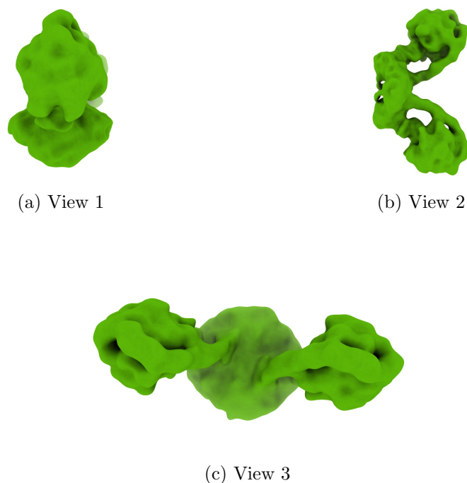
Figure 4: Isosurface at threshold=0.006640. Views generated by ChimeraX at a the following X, Y, Z angles: View 1 (0, -90, -90), View 2 (-90, 0, -90), View 3 (0, 0, 0).
