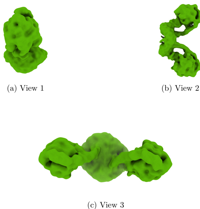
Figure 4: Isosurface at threshold=0.007180. Views generated by ChimeraX at a the following X, Y, Z angles: View 1 (0, -90, -90), View 2 (-90, 0, -90), View 3 (0, 0, 0).
