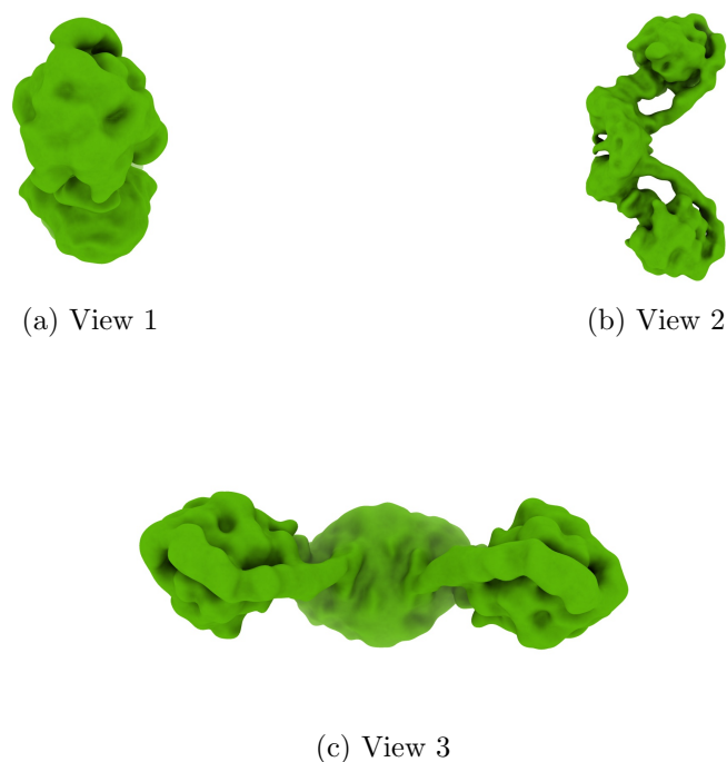
Figure 4: Isosurface at threshold=0.007390. Views generated by ChimeraX at a the following X, Y, Z angles: View 1 (0, -90, -90), View 2 (-90, 0, -90), View 3 (0, 0, 0).
