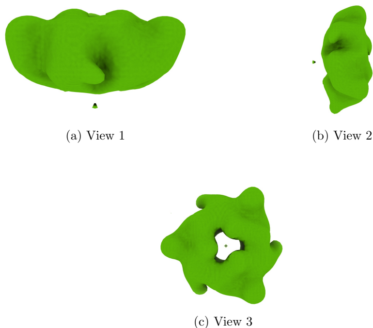
Figure 4: Isosurface at threshold=0.024400. Views generated by ChimeraX at a the following X, Y, Z angles: View 1 (0, -90, -90), View 2 (-90, 0, -90), View 3 (0, 0, 0).
