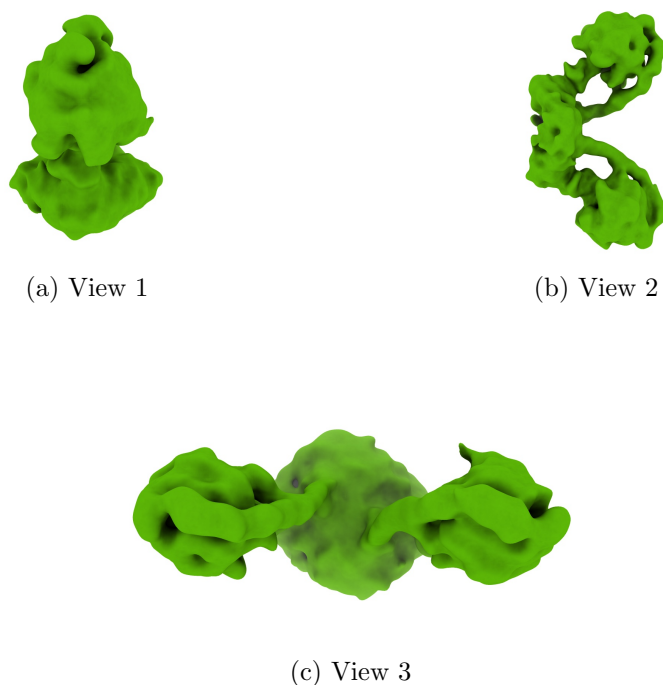
Figure 4: Isosurface at threshold=0.007210. Views generated by ChimeraX at a the following X, Y, Z angles: View 1 (0, -90, -90), View 2 (-90, 0, -90), View 3 (0, 0, 0).
