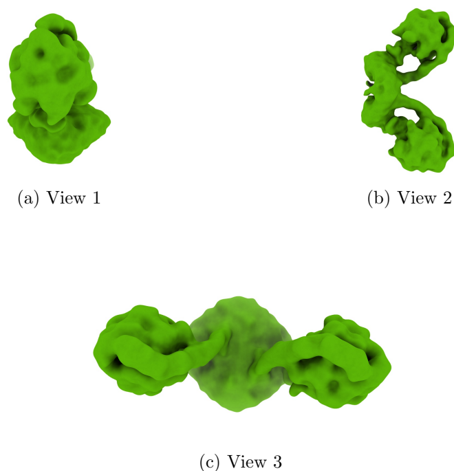
Figure 4: Isosurface at threshold=0.006910. Views generated by ChimeraX at a the following X, Y, Z angles: View 1 (0, -90, -90), View 2 (-90, 0, -90), View 3 (0, 0, 0).
