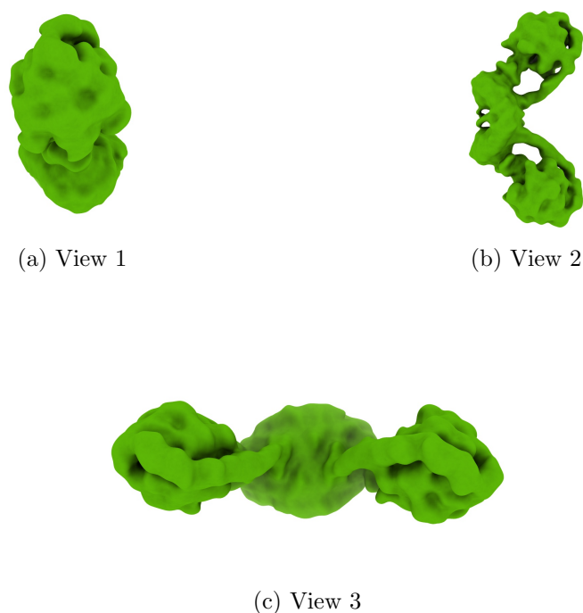
Figure 4: Isosurface at threshold=0.006940. Views generated by ChimeraX at a the following X, Y, Z angles: View 1 (0, -90, -90), View 2 (-90, 0, -90), View 3 (0, 0, 0).
