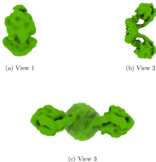
Figure 4: Isosurface at threshold=0.006680. Views generated by ChimeraX at a the following X, Y, Z angles: View 1 (0, -90, -90), View 2 (-90, 0, -90), View 3 (0, 0, 0).
