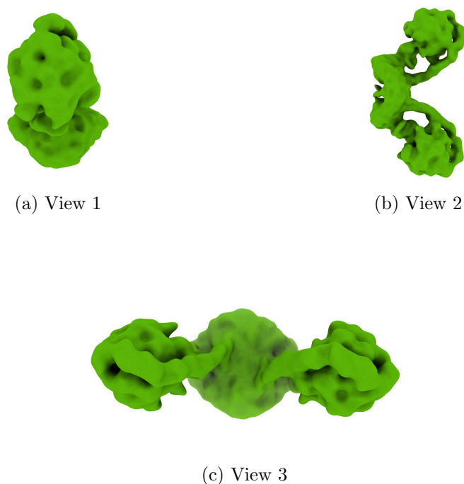
Figure 4: Isosurface at threshold=0.007740. Views generated by ChimeraX at a the following X, Y, Z angles: View 1 (0, -90, -90), View 2 (-90, 0, -90), View 3 (0, 0, 0).
