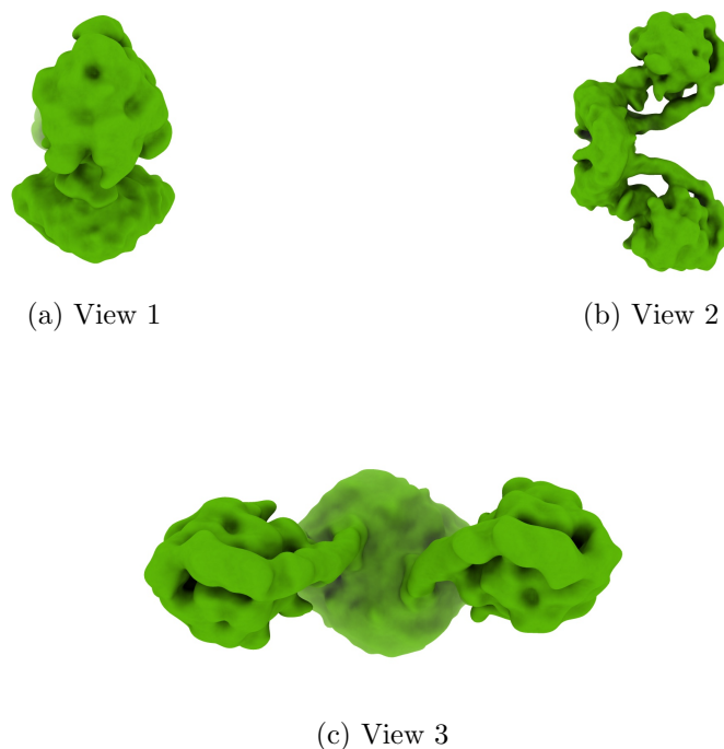
Figure 4: Isosurface at threshold=0.006690. Views generated by ChimeraX at a the following X, Y, Z angles: View 1 (0, -90, -90), View 2 (-90, 0, -90), View 3 (0, 0, 0).
