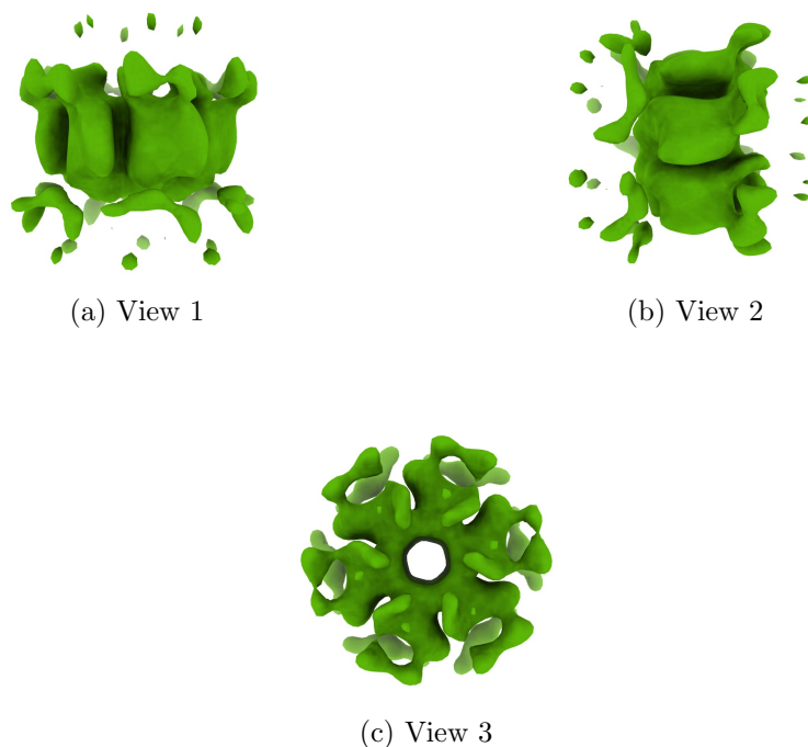
Figure 4: Isosurface at threshold=0.002390. Views generated by ChimeraX at a the following X, Y, Z angles: View 1 (0, -90, -90), View 2 (-90, 0, -90), View 3 (0, 0, 0).
