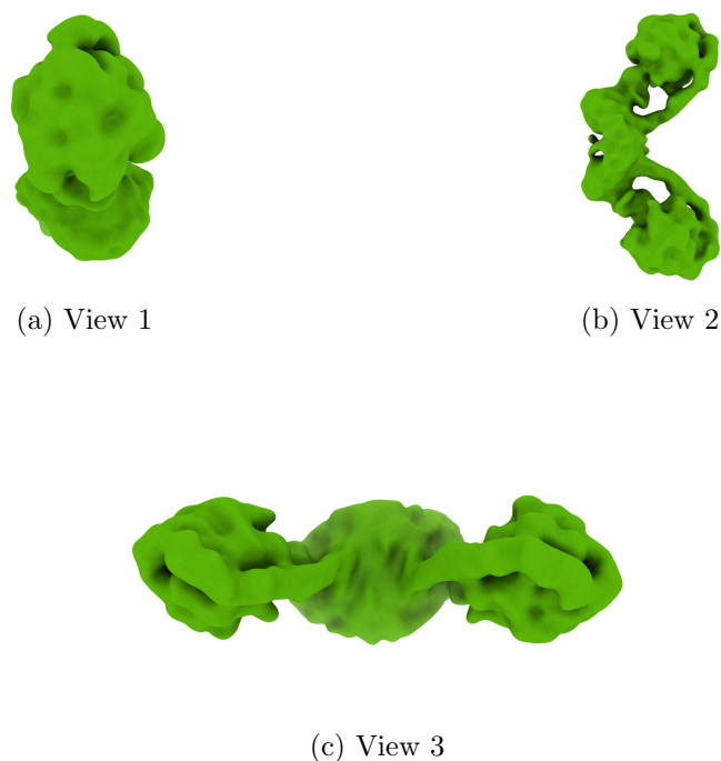
Figure 4: Isosurface at threshold=0.006850. Views generated by ChimeraX at a the following X, Y, Z angles: View 1 (0, -90, -90), View 2 (-90, 0, -90), View 3 (0, 0, 0).
