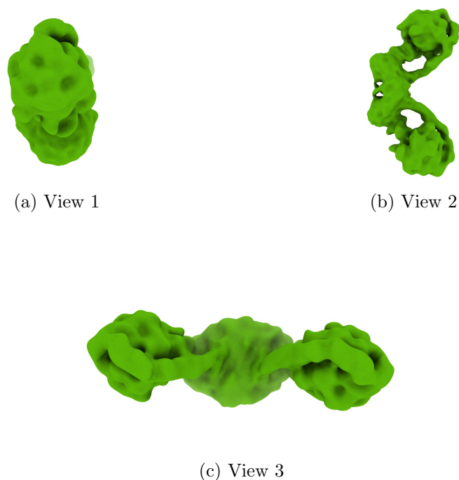
Figure 4: Isosurface at threshold=0.007130. Views generated by ChimeraX at a the following X, Y, Z angles: View 1 (0, -90, -90), View 2 (-90, 0, -90), View 3 (0, 0, 0).
