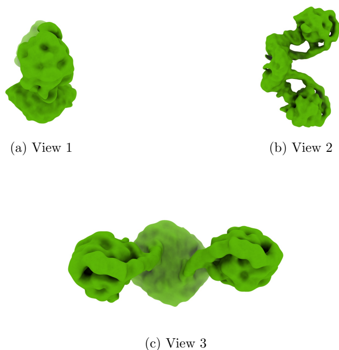
Figure 4: Isosurface at threshold=0.007890. Views generated by ChimeraX at a the following X, Y, Z angles: View 1 (0, -90, -90), View 2 (-90, 0, -90), View 3 (0, 0, 0).
