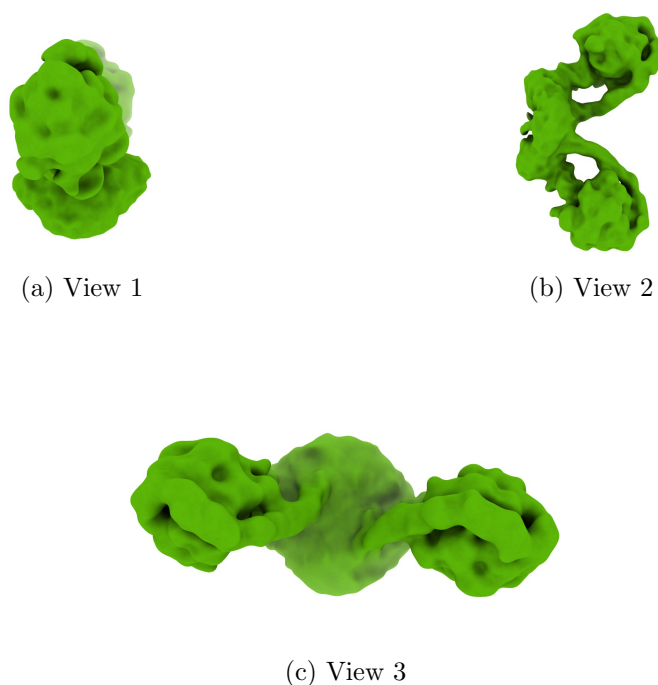
Figure 4: Isosurface at threshold=0.006750. Views generated by ChimeraX at a the following X, Y, Z angles: View 1 (0, -90, -90), View 2 (-90, 0, -90), View 3 (0, 0, 0).
