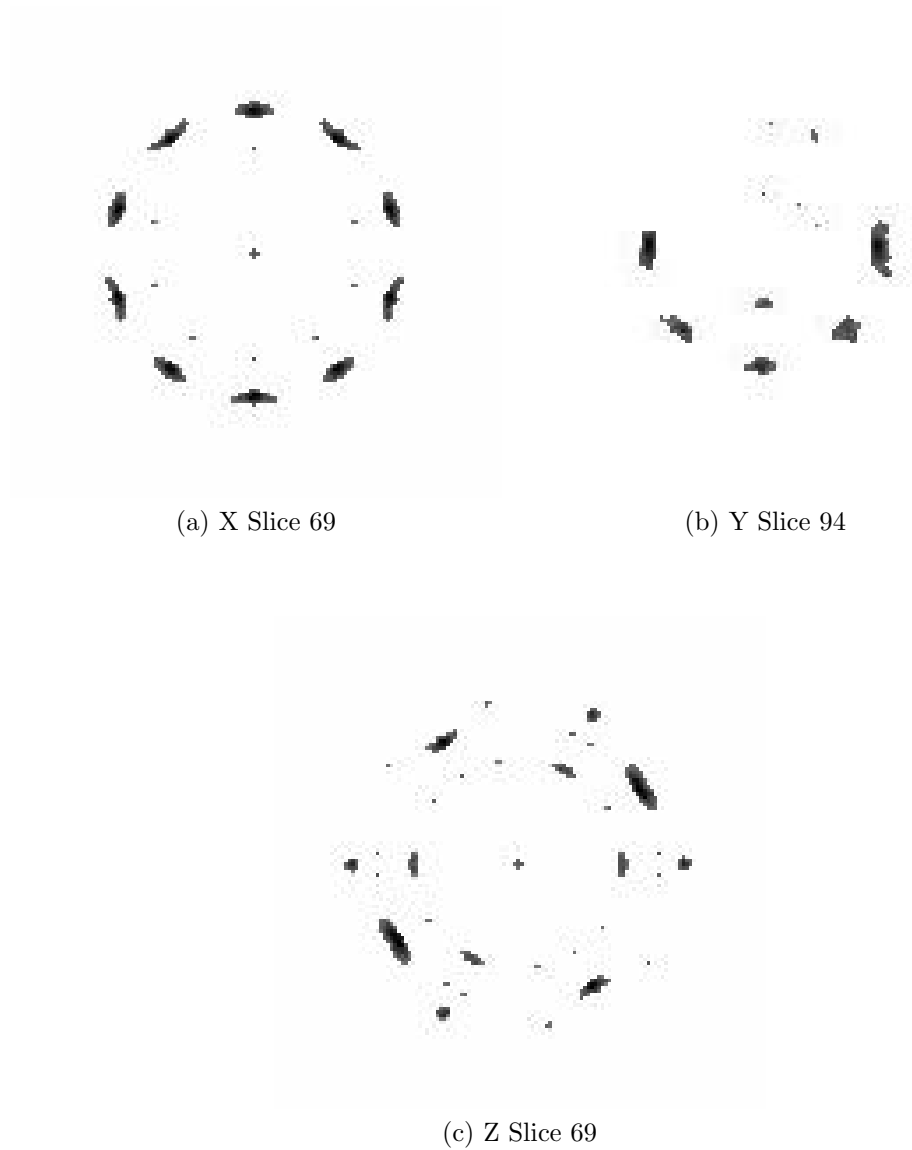
Figure 9: Maximum variance slices in the three dimensions of the parts of the background beyond 5\sigma
