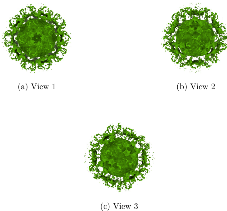
Figure 4: Isosurface at threshold=0.639000. Views generated by ChimeraX at a the following X, Y, Z angles: View 1 (0, -90, -90), View 2 (-90, 0, -90), View 3 (0, 0, 0).
