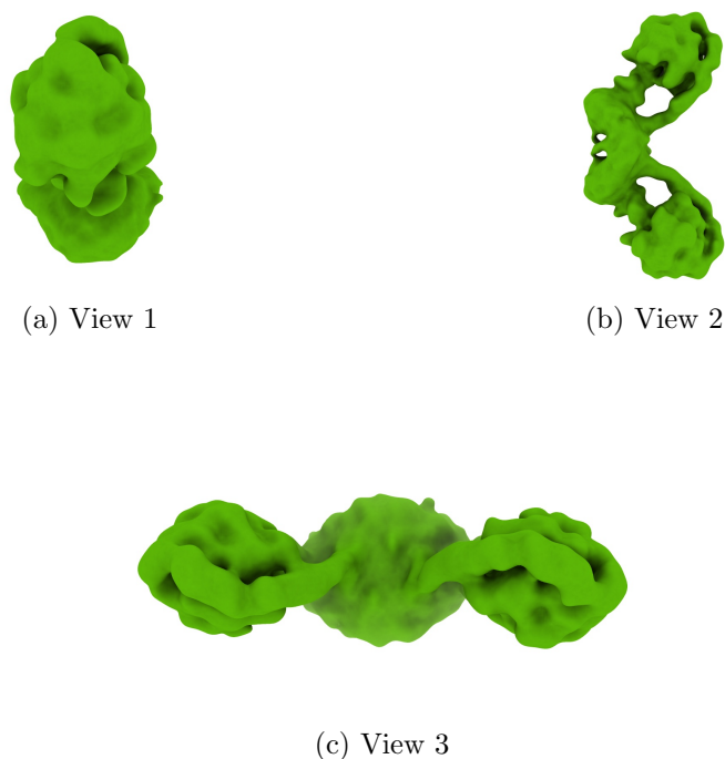
Figure 4: Isosurface at threshold=0.006740. Views generated by ChimeraX at a the following X, Y, Z angles: View 1 (0, -90, -90), View 2 (-90, 0, -90), View 3 (0, 0, 0).
