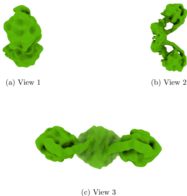
Figure 4: Isosurface at threshold=0.006700. Views generated by ChimeraX at a the following X, Y, Z angles: View 1 (0, -90, -90), View 2 (-90, 0, -90), View 3 (0, 0, 0).
