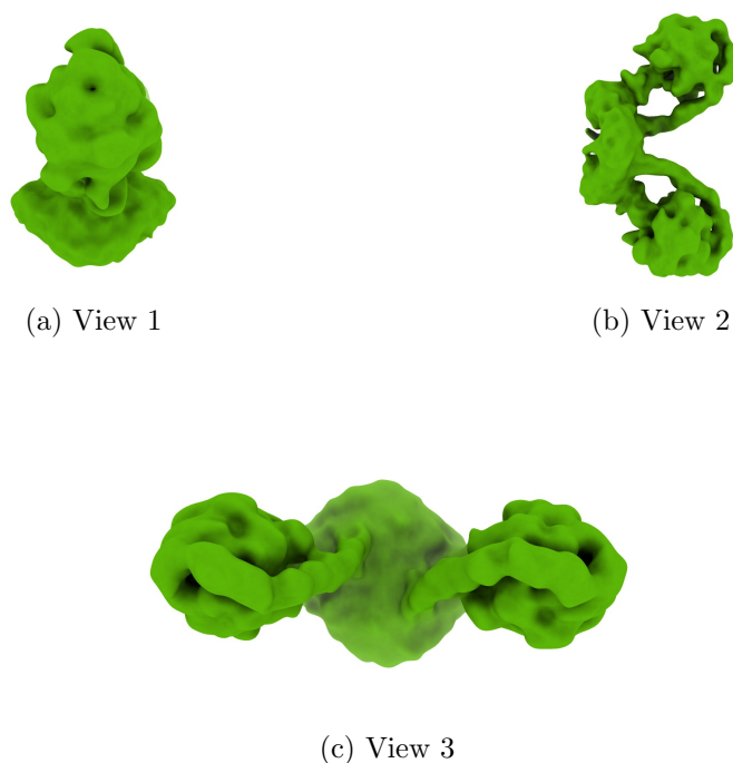
Figure 4: Isosurface at threshold=0.007670. Views generated by ChimeraX at a the following X, Y, Z angles: View 1 (0, -90, -90), View 2 (-90, 0, -90), View 3 (0, 0, 0).
