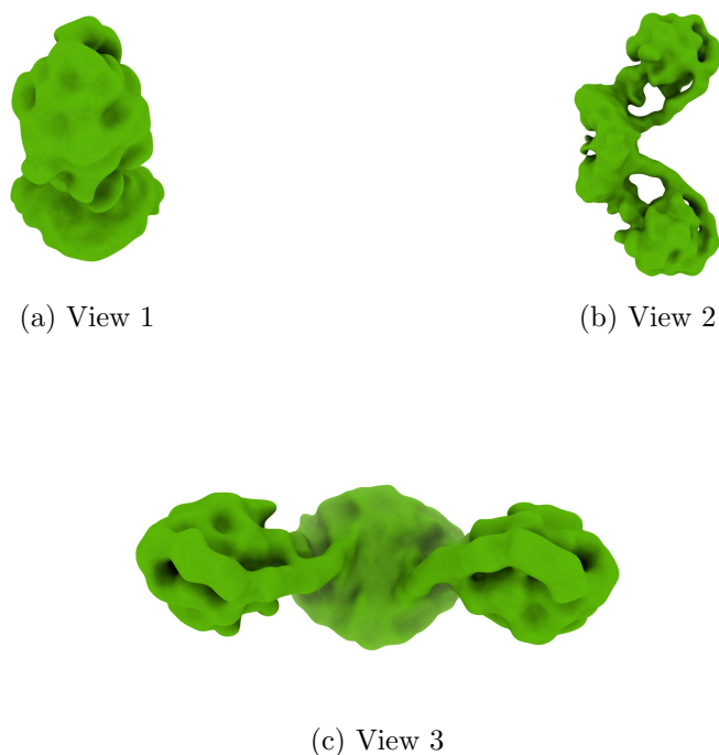
Figure 4: Isosurface at threshold=0.006930. Views generated by ChimeraX at a the following X, Y, Z angles: View 1 (0, -90, -90), View 2 (-90, 0, -90), View 3 (0, 0, 0).
