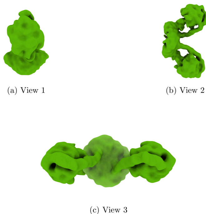
Figure 4: Isosurface at threshold=0.007100. Views generated by ChimeraX at a the following X, Y, Z angles: View 1 (0, -90, -90), View 2 (-90, 0, -90), View 3 (0, 0, 0).
