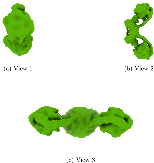
Figure 4: Isosurface at threshold=0.006070. Views generated by ChimeraX at a the following X, Y, Z angles: View 1 (0, -90, -90), View 2 (-90, 0, -90), View 3 (0, 0, 0).
