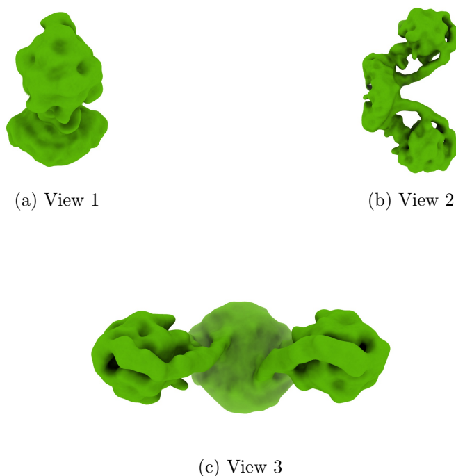
Figure 4: Isosurface at threshold=0.007450. Views generated by ChimeraX at a the following X, Y, Z angles: View 1 (0, -90, -90), View 2 (-90, 0, -90), View 3 (0, 0, 0).
